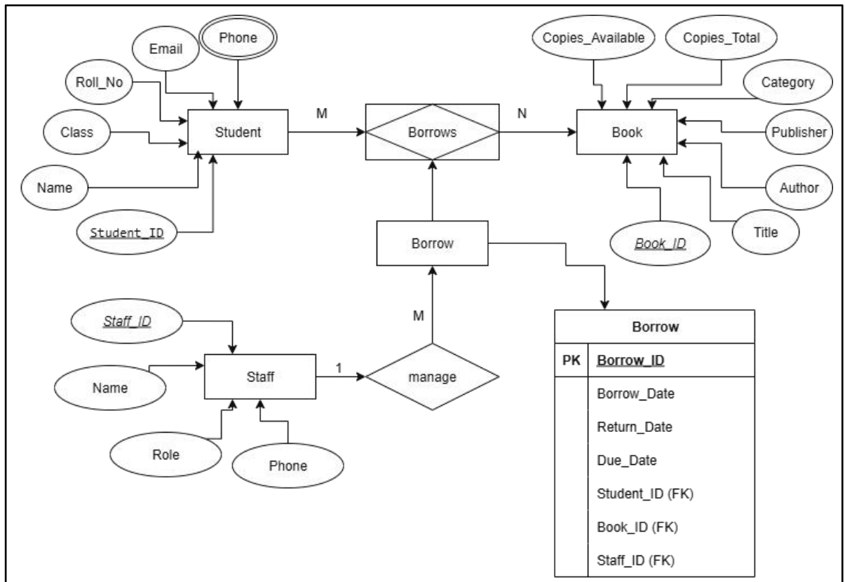
Fig: ER diagram of Library System
